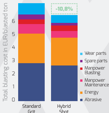
Total blasting cost Standard Grit vs. Hybrid Shot
